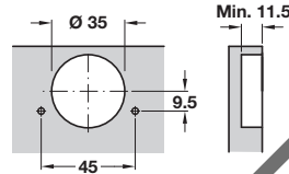
Drilling pattern for cup fixing
