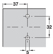
With pre-mounted Euro screws
